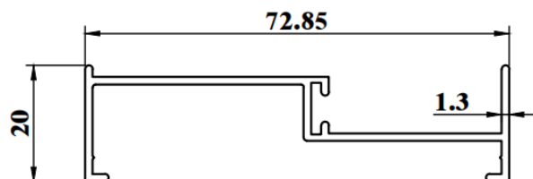
ESD170HH WEIGHT : 0.461 KG/M AP : 264.61mm
