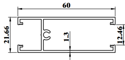
ESD178H WEIGHT : 0.587 KG/M AP : 340.28mm
