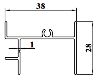
ESD172C WEIGHT : 0.293 KG/M AP : 210.73mm
