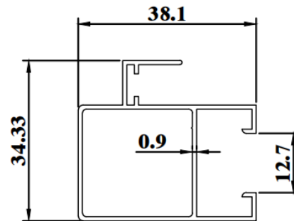
ESD174A WEIGHT : 0.395 KG/M AP : 228.54mm
