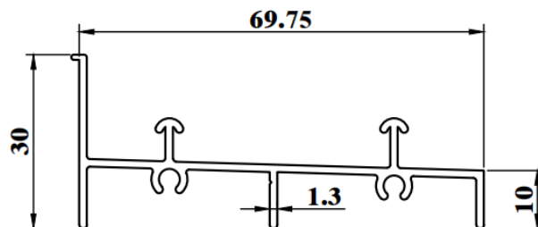
ESD175HB WEIGHT : 0.565 KG/M AP : 312.52mm
